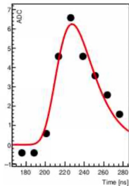
Example of a 1PE dark noise pulse
